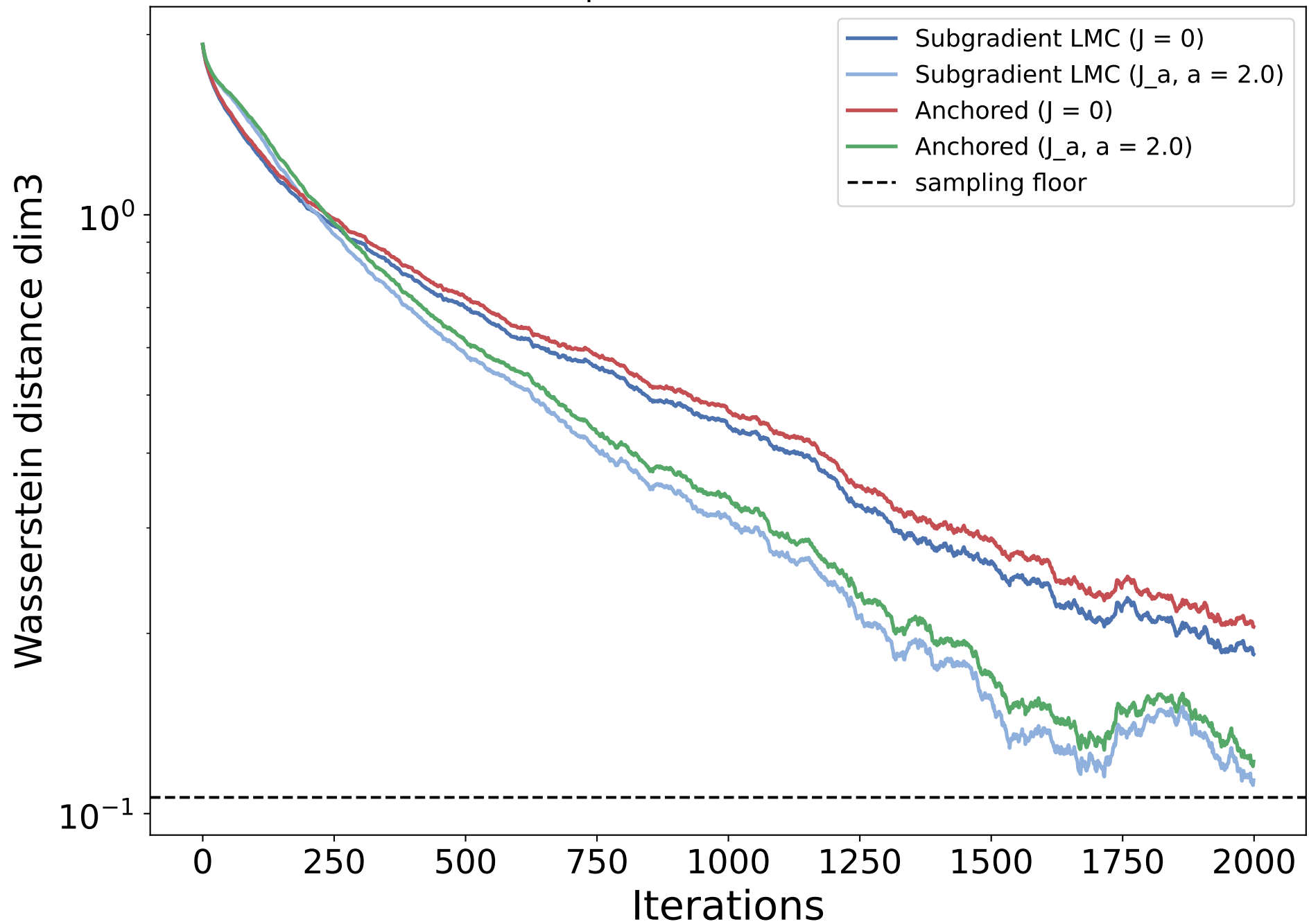
Product Laplace, coordinate 3 ( b = 2.0 )
