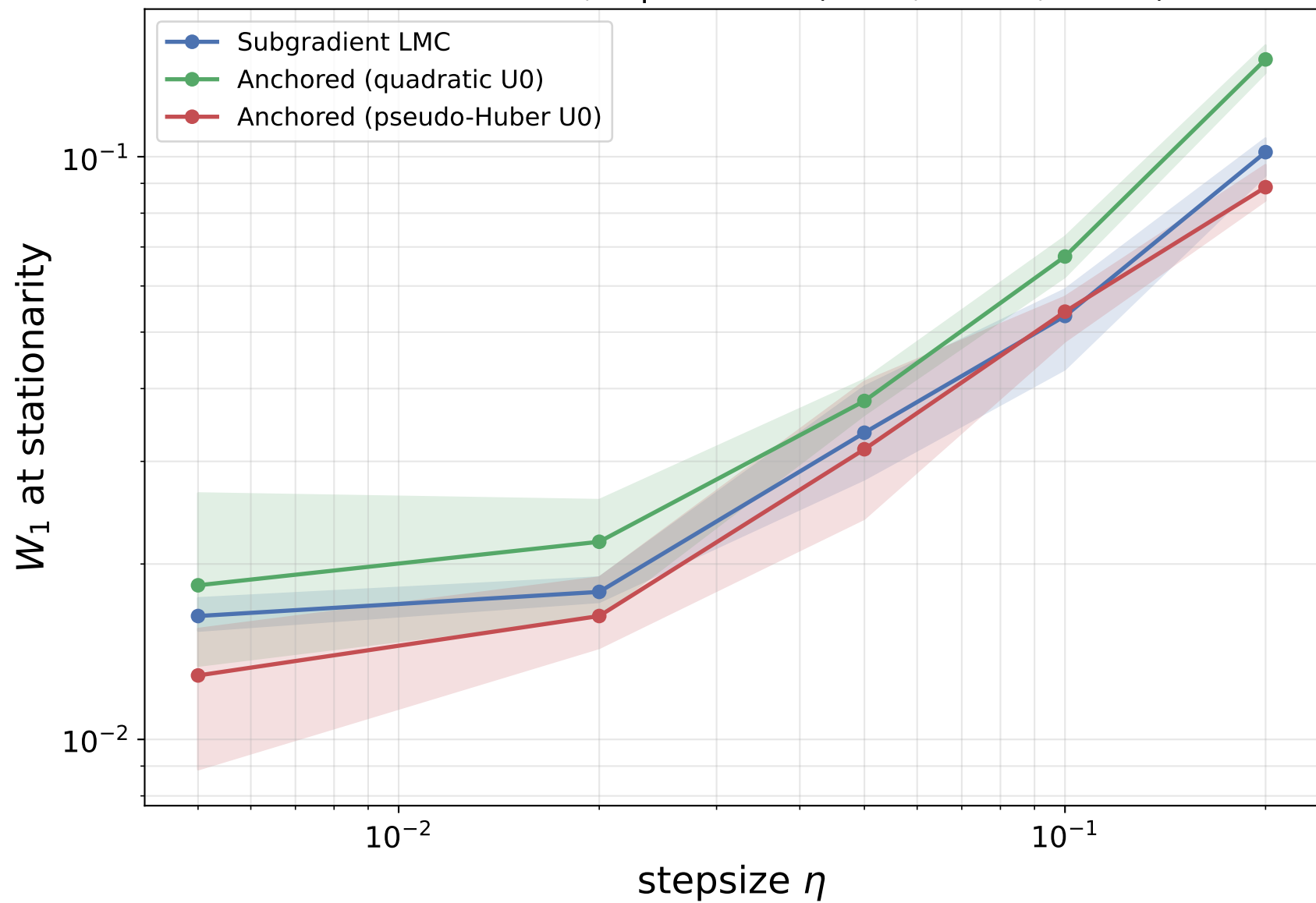
Discretization bias, Laplace on R ( b = 1 , T = 50 , 3 runs)
