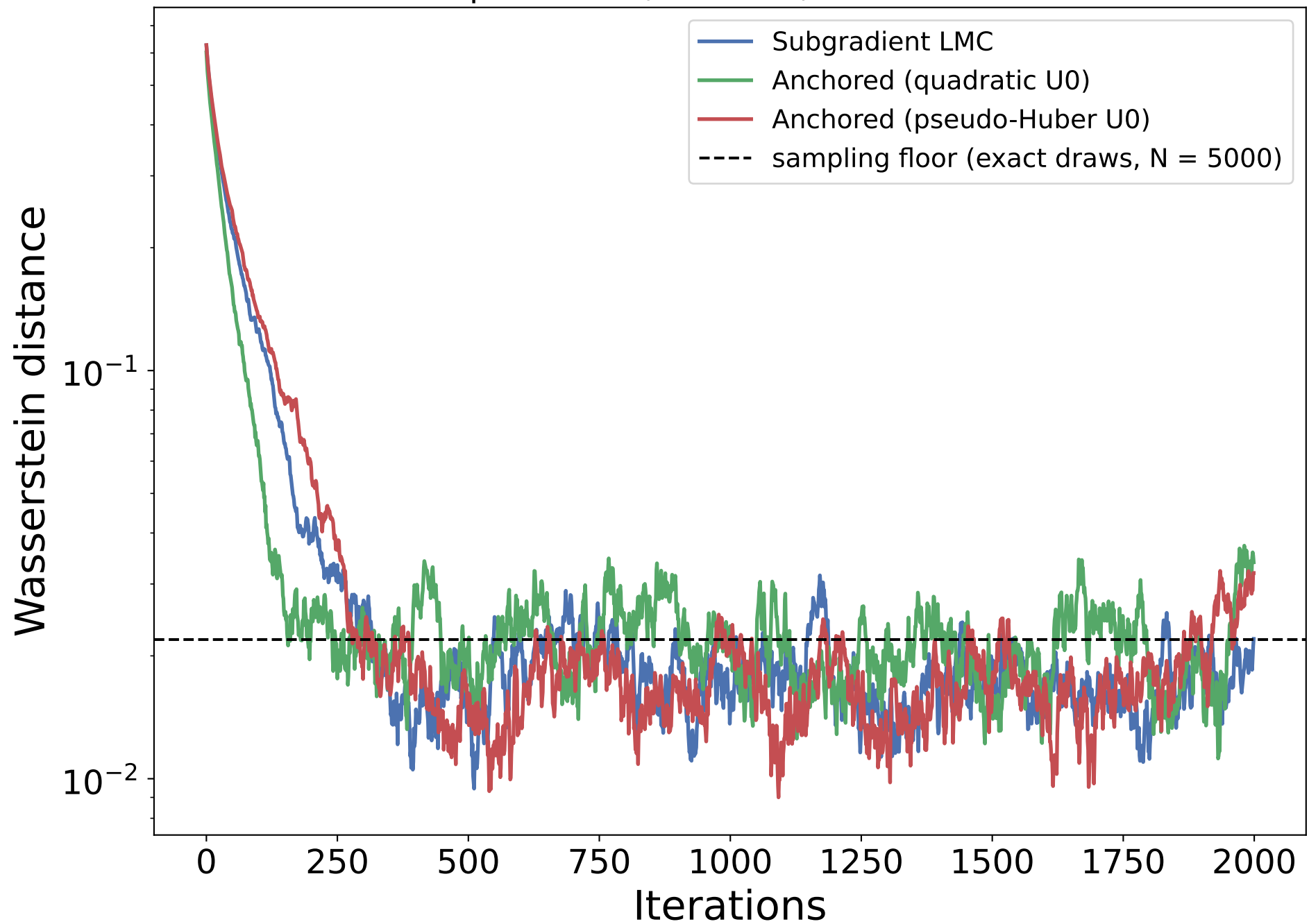
Laplace on R, b = 0.5 , \eta = 0.005
