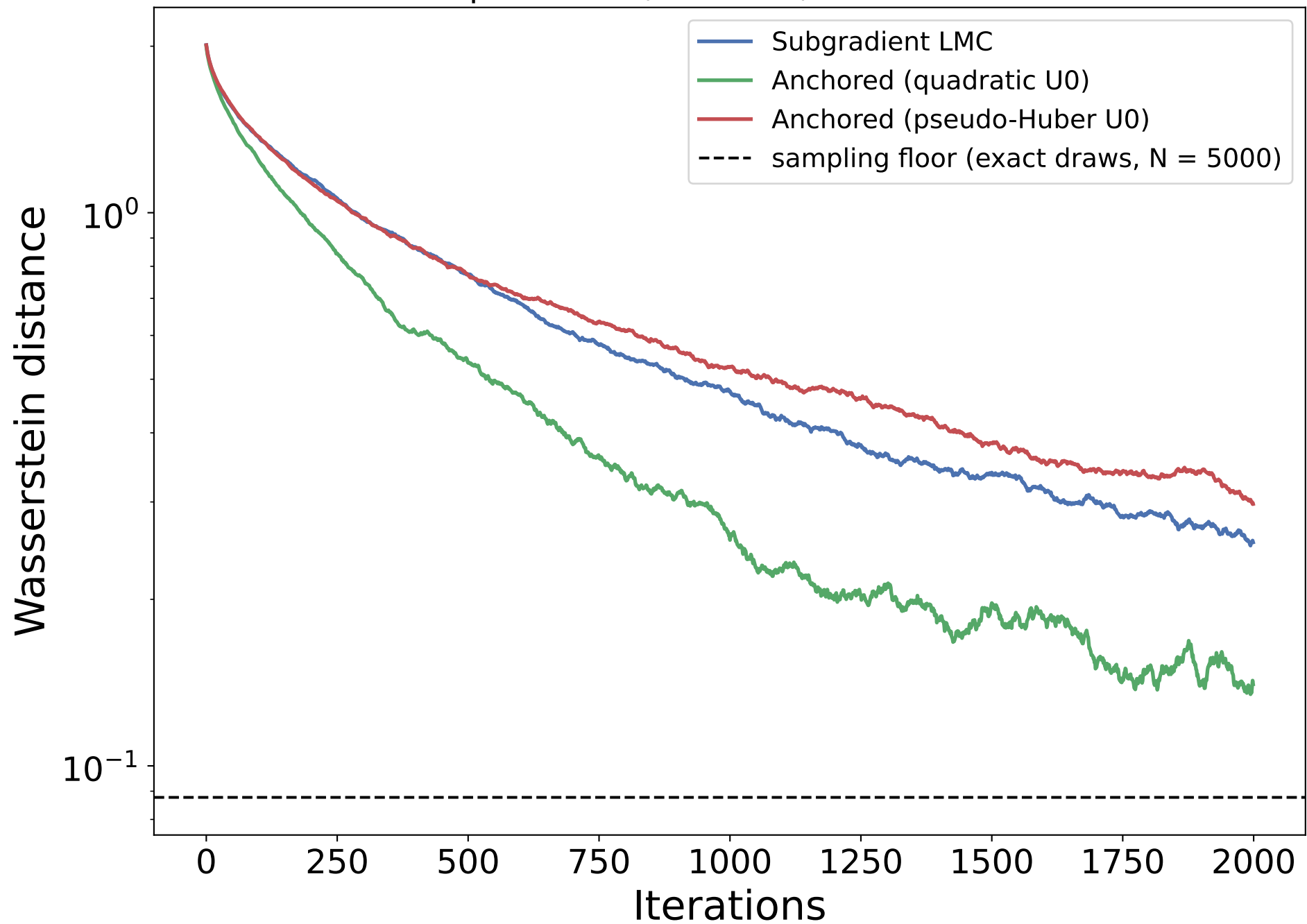
Laplace on R, b = 2.0 , \eta = 0.005
