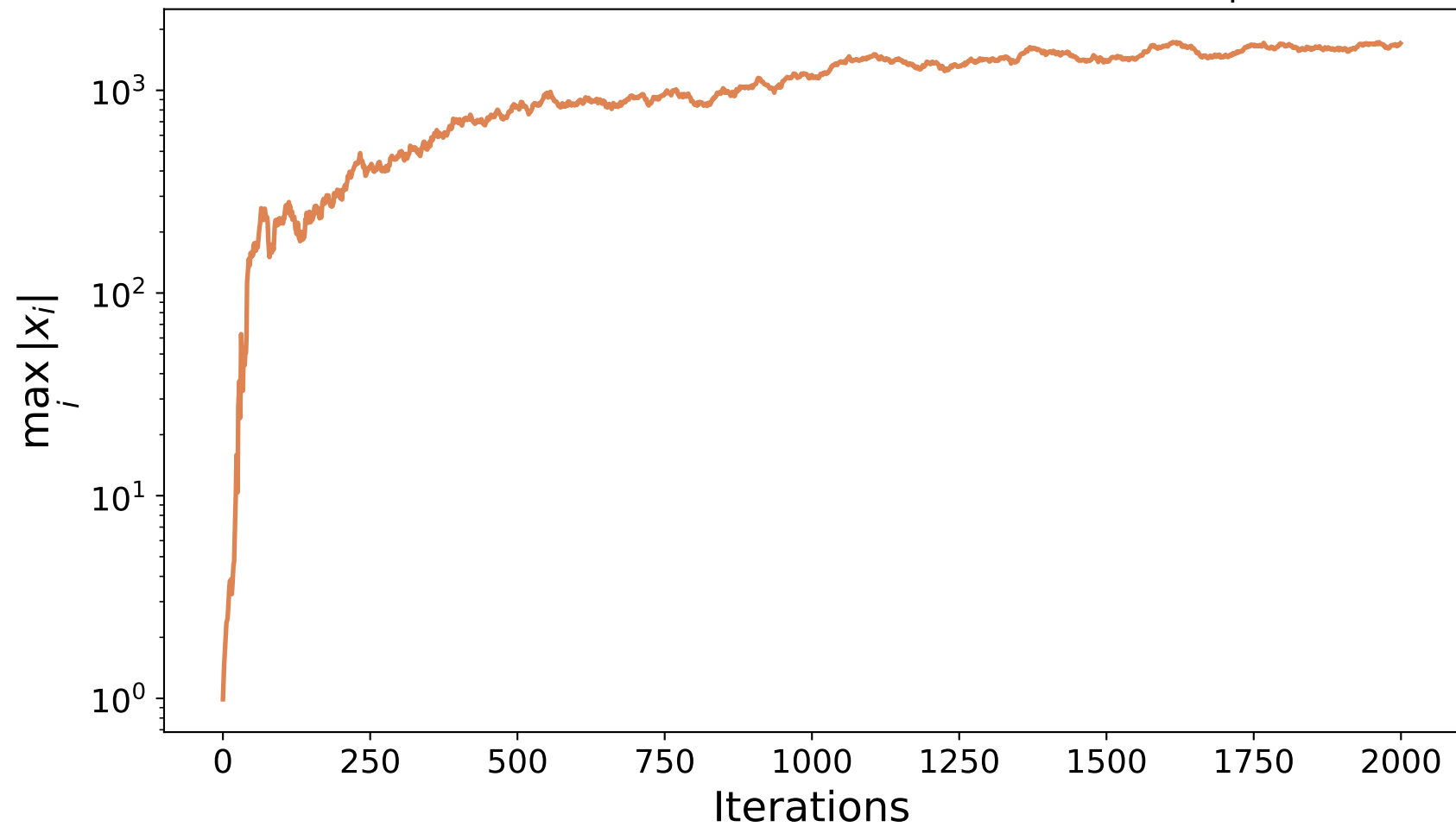
Zero anchor on the unbounded line: ensemble escapes
