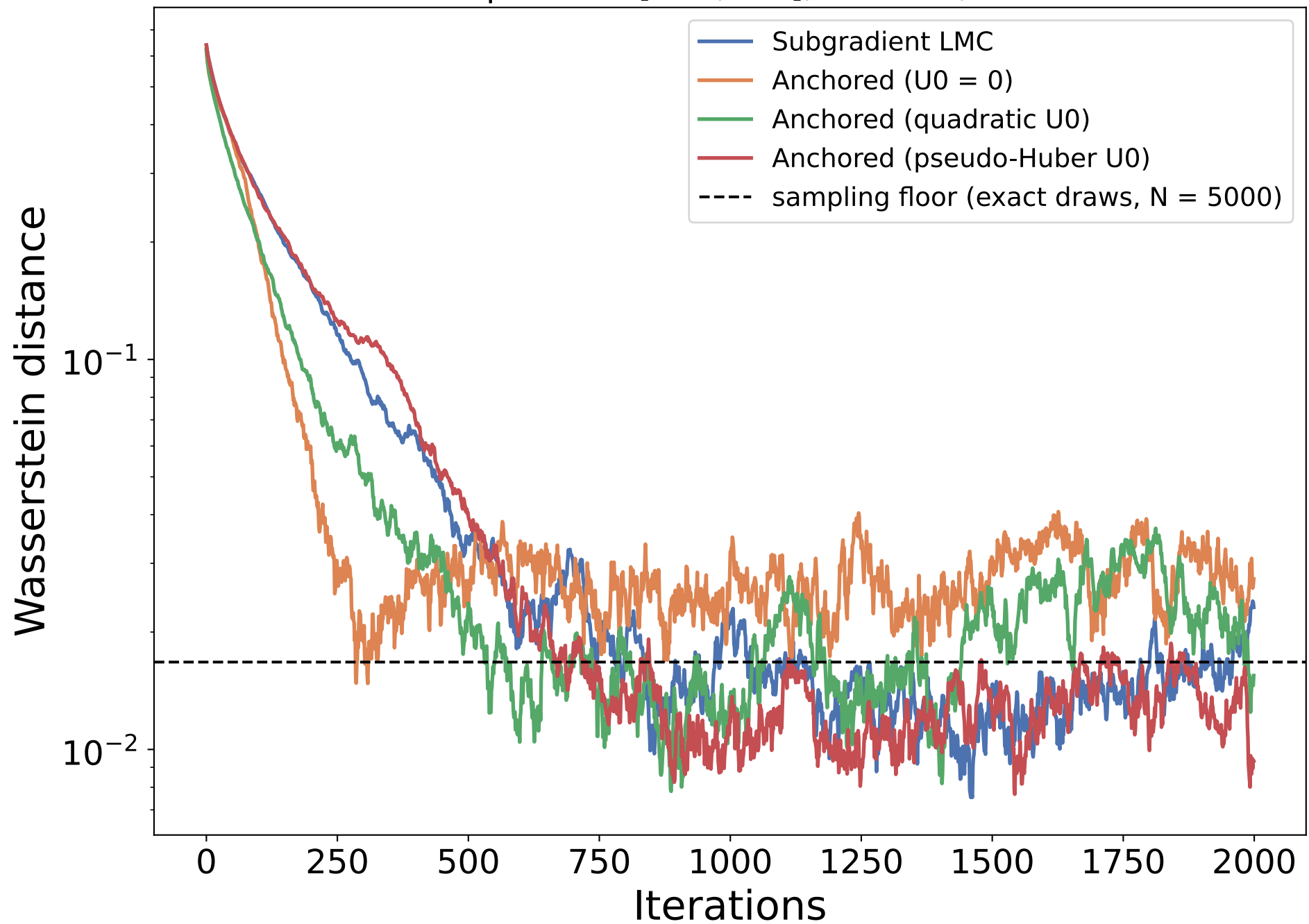
Truncated Laplace on [-3.0, 3.0] , b = 0.5 , \eta = 0.002
