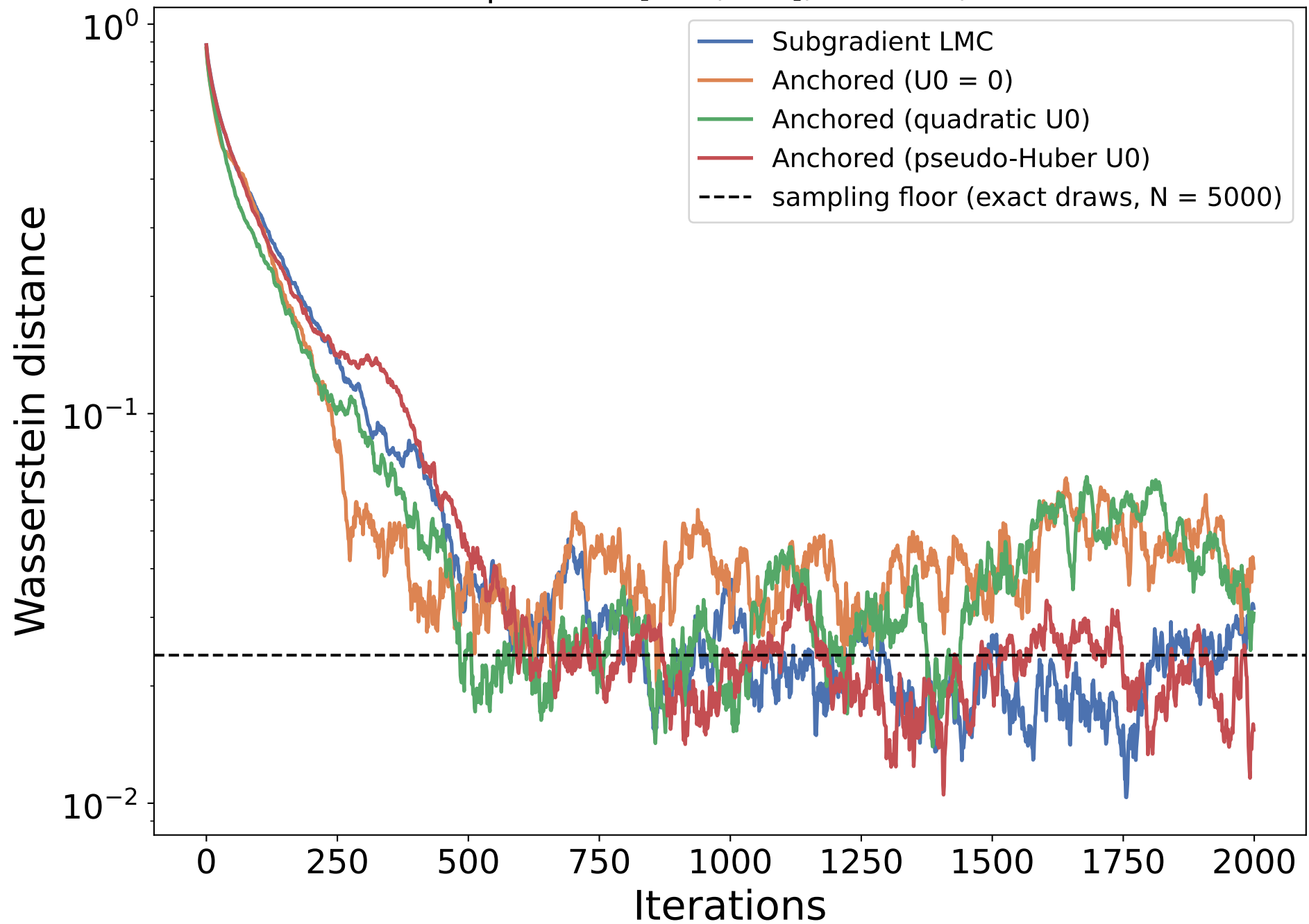
Truncated Laplace on [-3.0, 3.0] , b = 1.0 , \eta = 0.005
