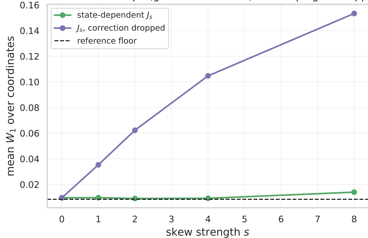
MAGIC Gamma Telescope (gamma vs hadron) — keeping vs dropping \nabla \cdot J
