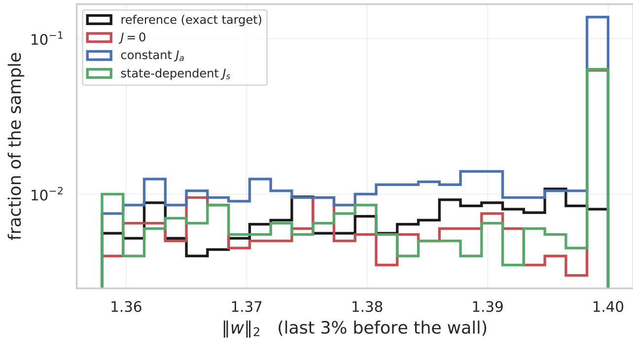
the projection atom at \|w\| = R
