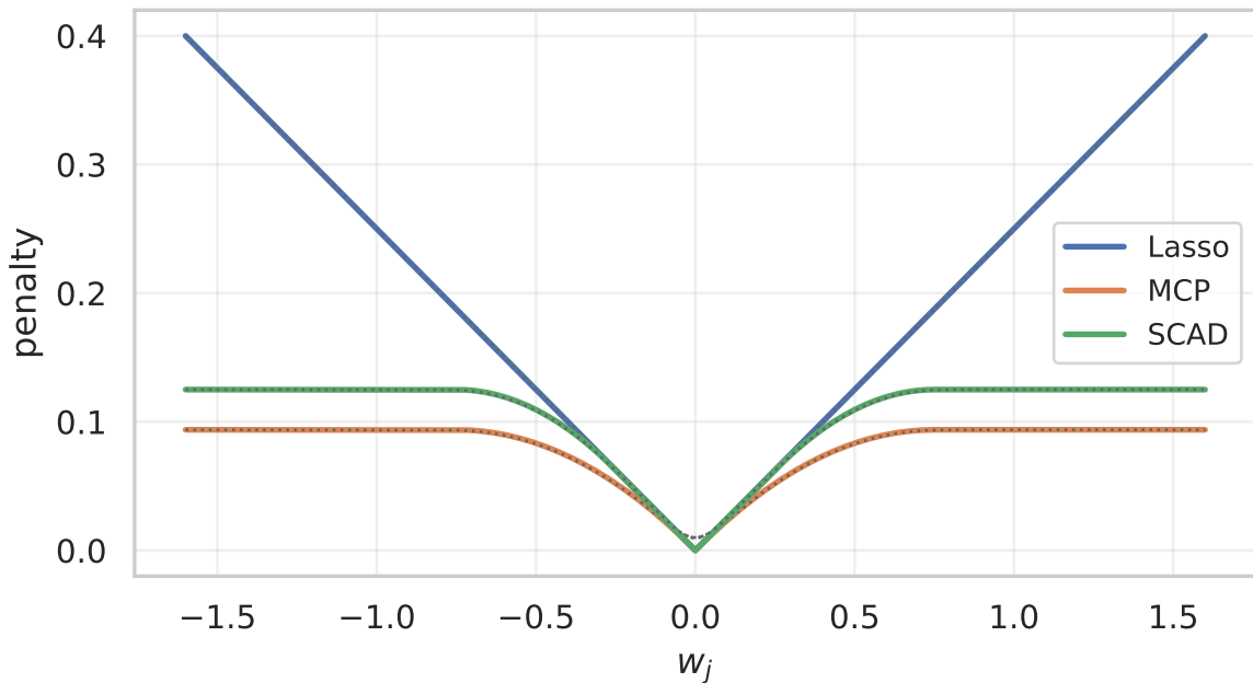
The three regularizers at \lambda = 0.25 , a = 3 (dotted: the Gaussian anchor p_0 )
