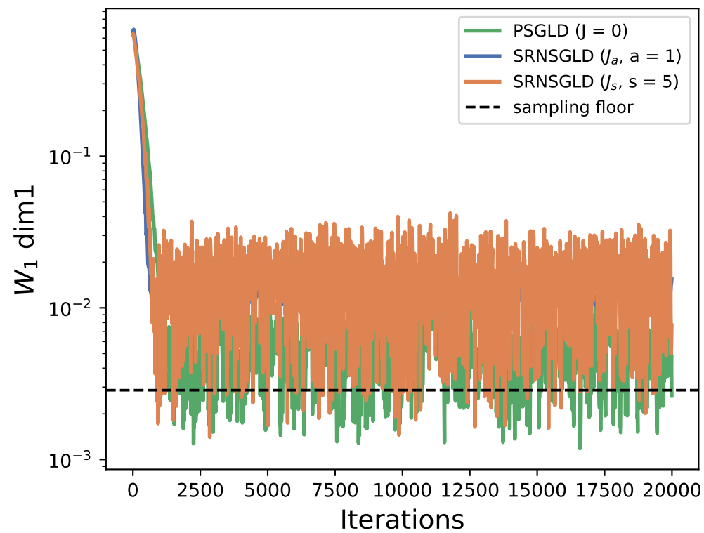
coordinate 1
