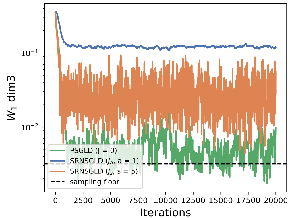
coordinate 3
