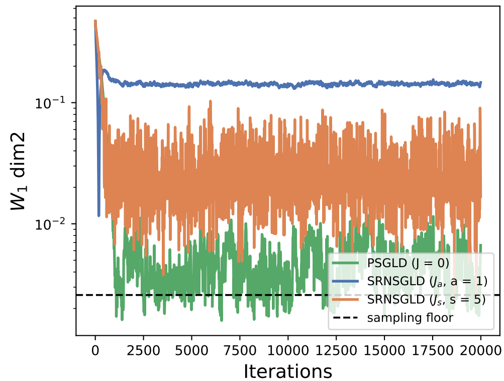
coordinate 2
