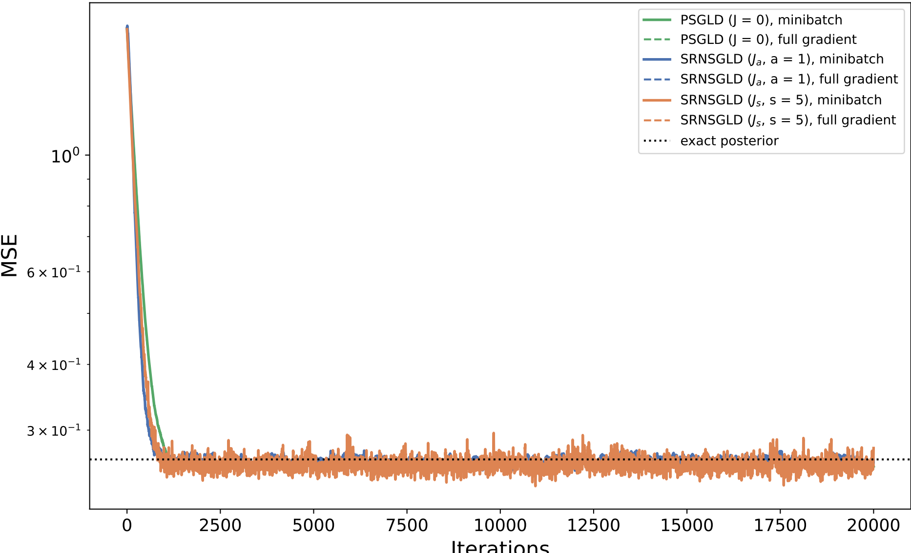
Minibatch ( m = 50 ) vs full gradient
