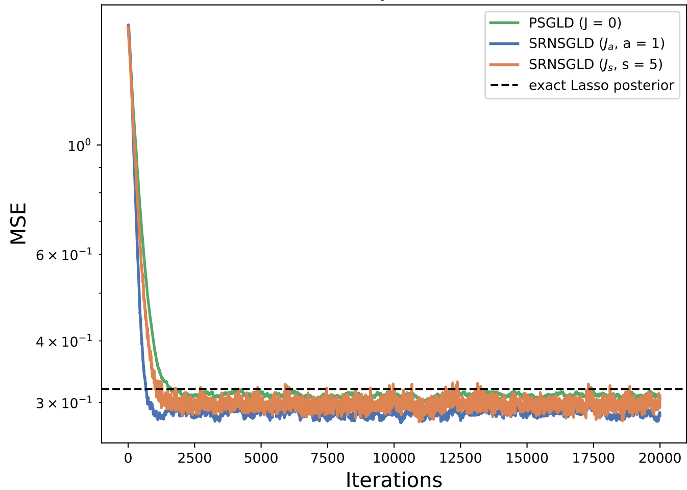
Constrained Bayesian Lasso: MSE
