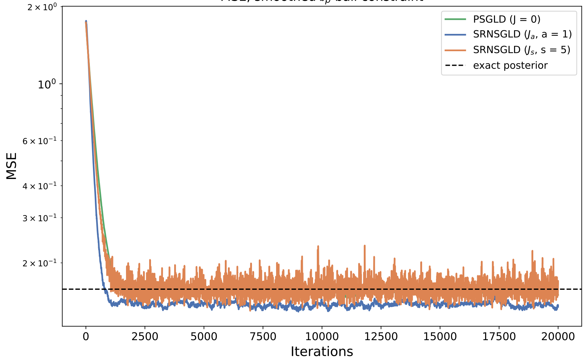
MSE, smoothed \ell_p ball constraint
