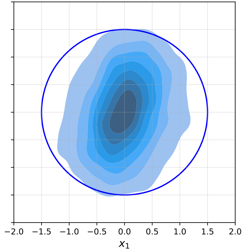
original: Euler + projection, j = 0 on boundary: 7.5%
