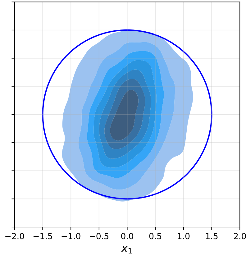
original + J_s , s = 4 on boundary: 7.8%
