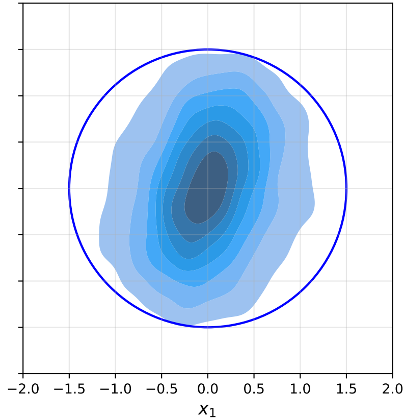
+ rotation + reflection + annealed J_s on boundary: 0.3%
