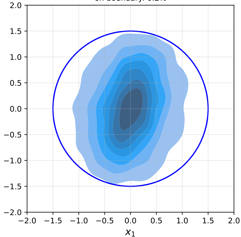
Target (rejection) on boundary: 0.2%
