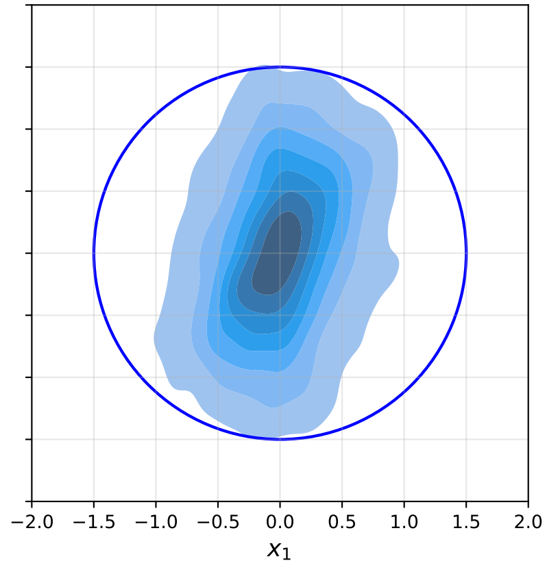
original: Euler + projection, J = 0 on boundary: 5.6%
