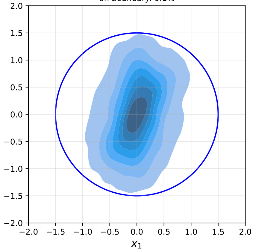
Target (rejection) on boundary: 0.1%
