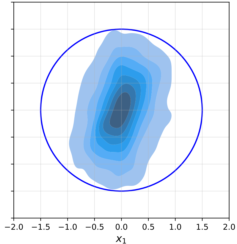
+ rotation + reflection + annealed J_s on boundary: 0.1%
