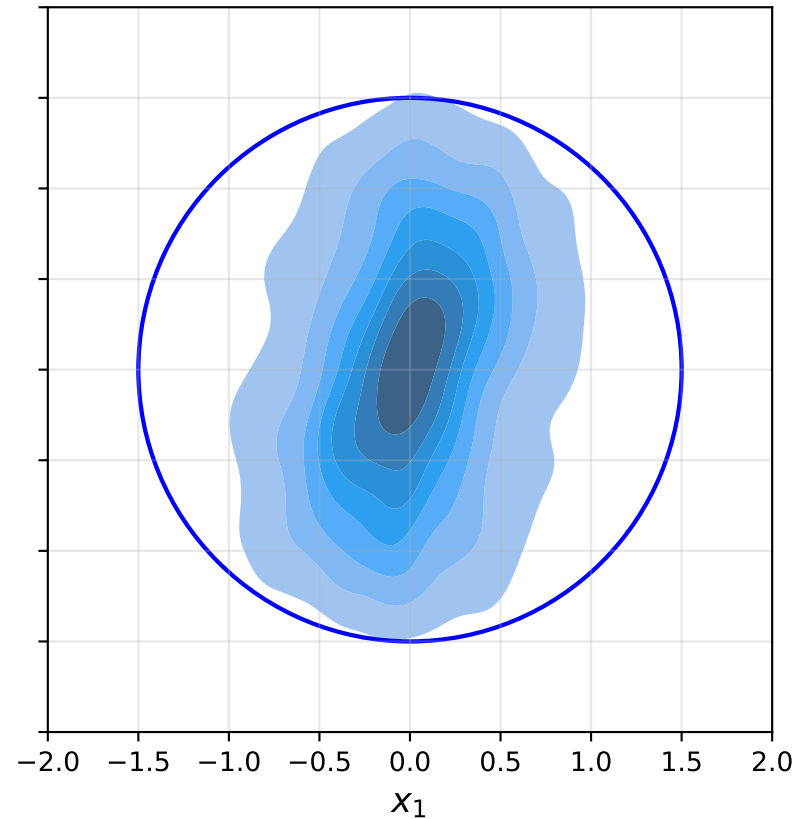
original + J_s , s = 4 on boundary: 6.4%
