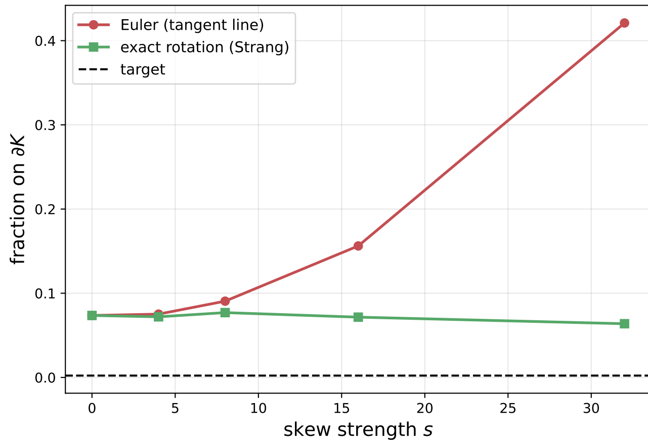
Euler leaks mass into the wall; the exact rotation does not
