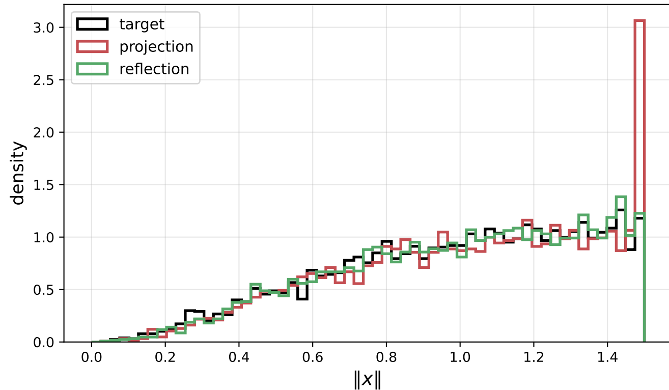
Target A: elliptical Laplace on K
