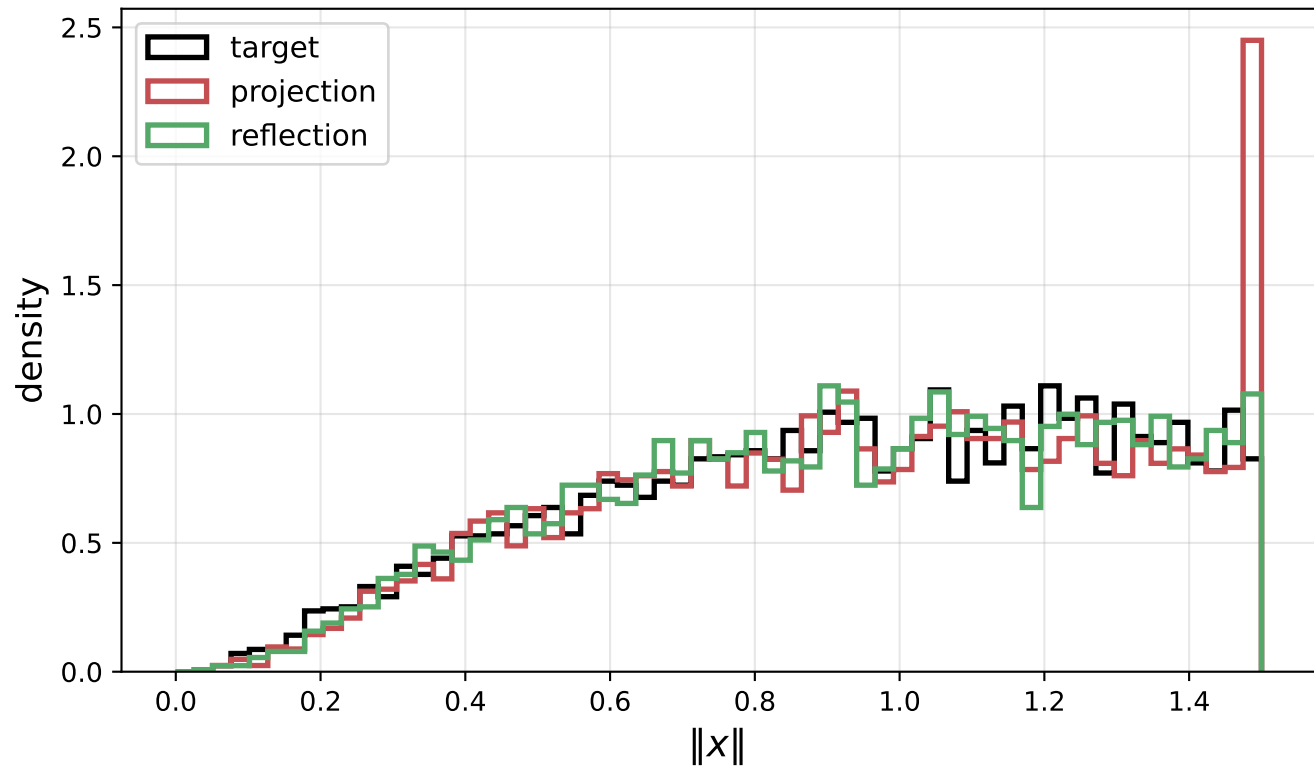
Target B: correlated \ell_1 Laplace on K
