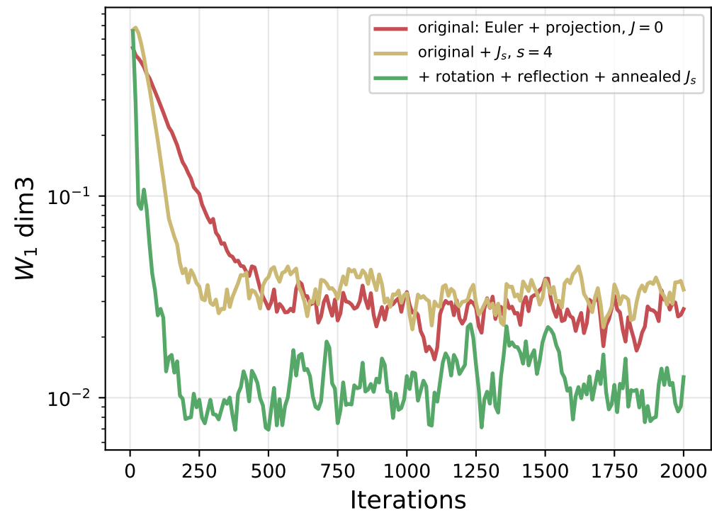
coordinate 3
