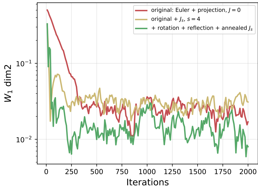
coordinate 2
