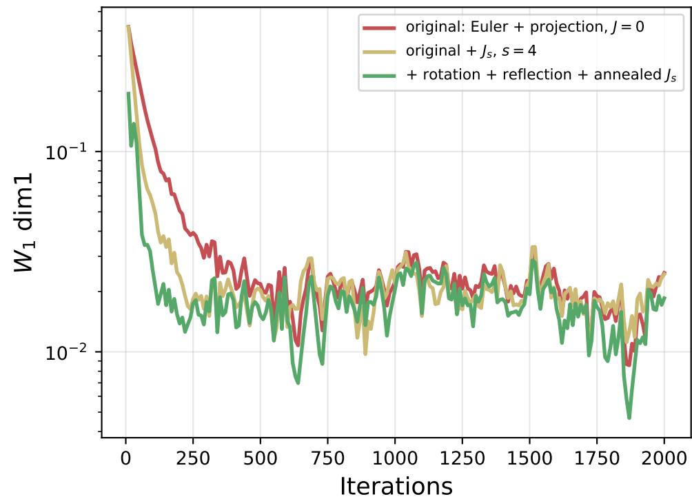
coordinate 1
