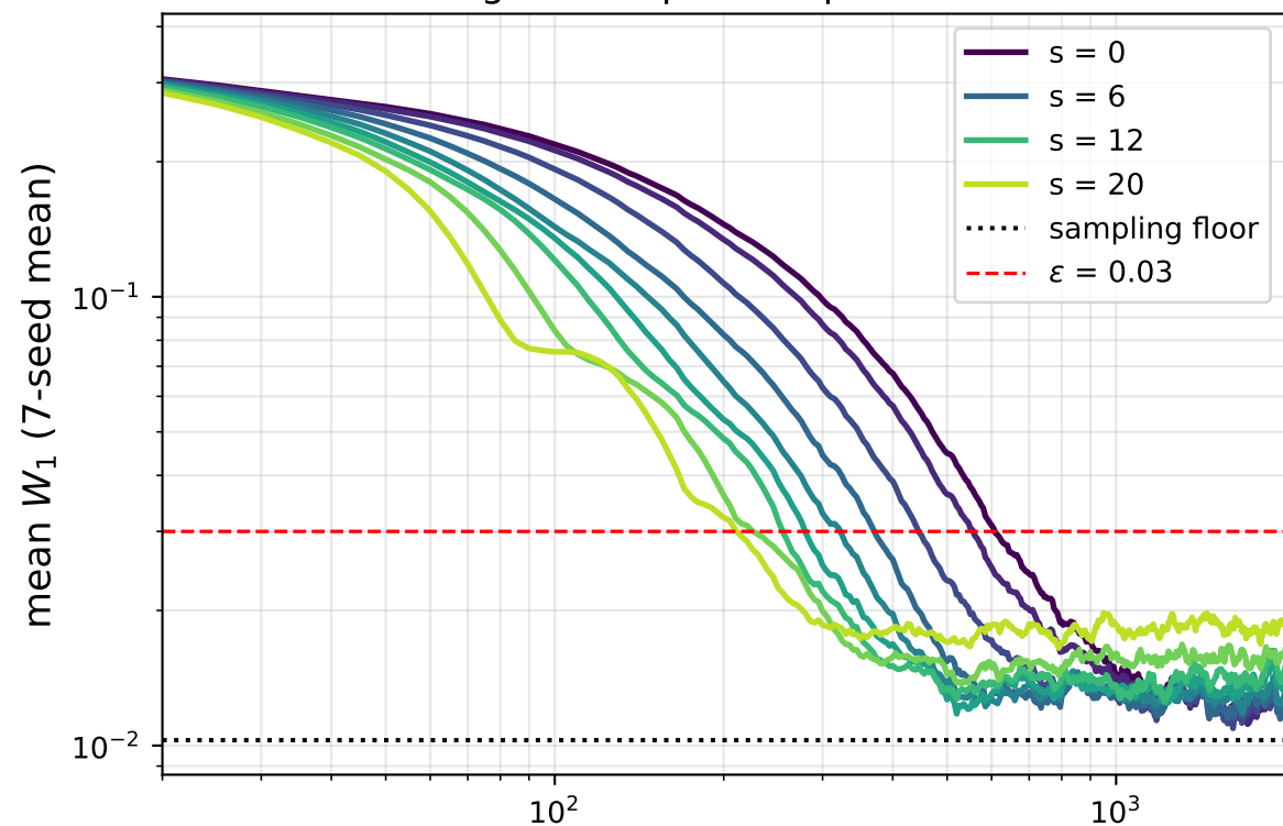
Target A: elliptical Laplace on K
