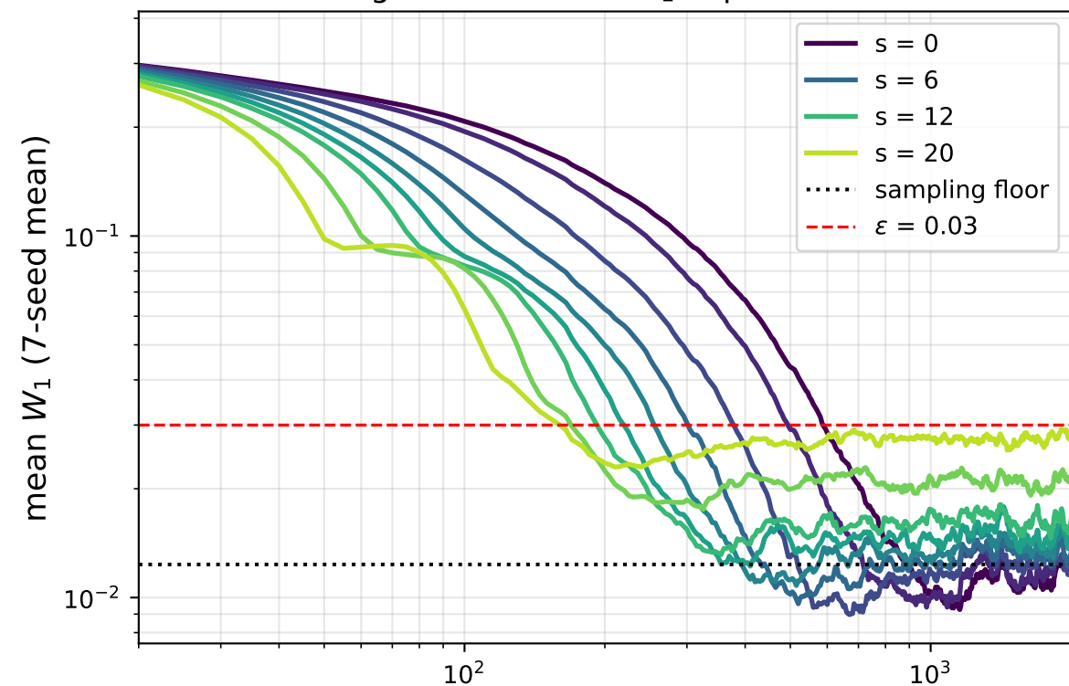
Target B: correlated \ell_1 Laplace on K
