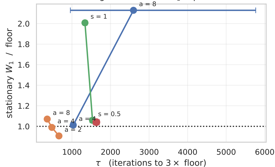
Target B: correlated \ell_1 Laplace
