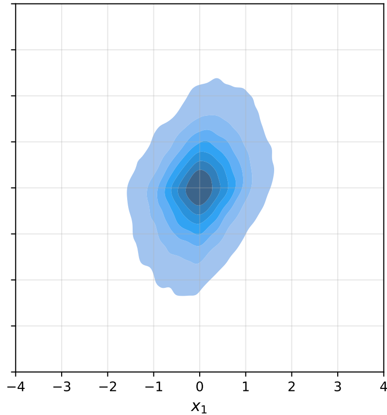
J = 0 (n = 48,000)
