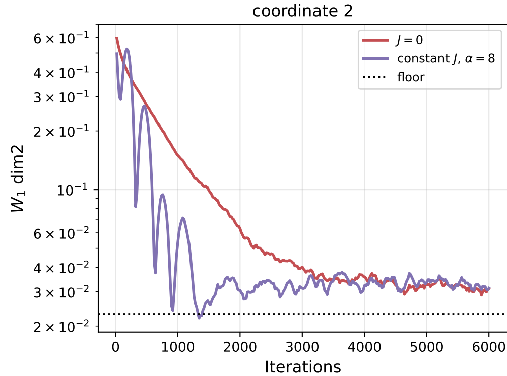
Lasso (unconstrained) — J = 0 vs constant J
