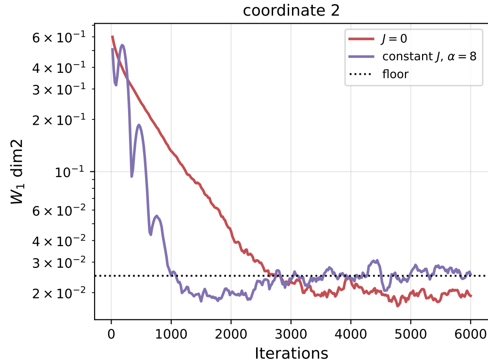
SCAD (unconstrained) — J = 0 vs constant J
