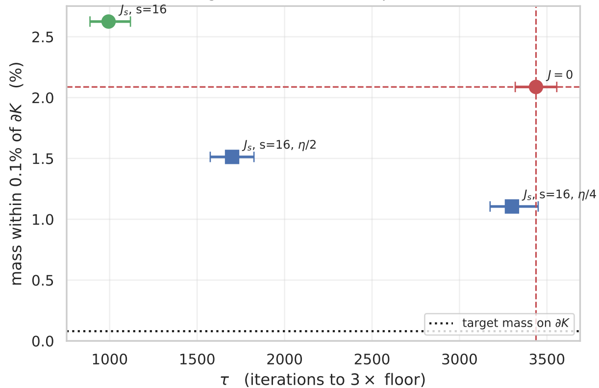
Target B: correlated \ell_1 Laplace on K
