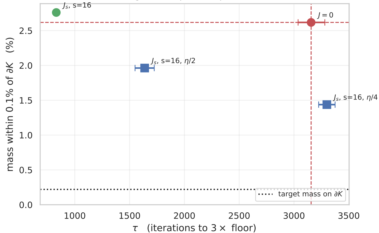
Target A: elliptical Laplace on K
