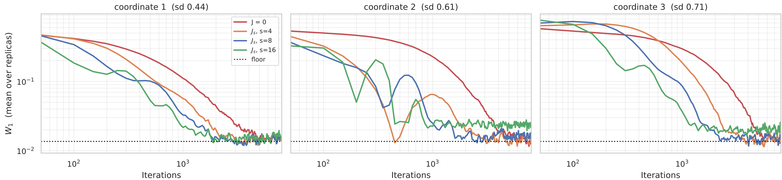
Target A: elliptical Laplace on K — W_1 per coordinate
