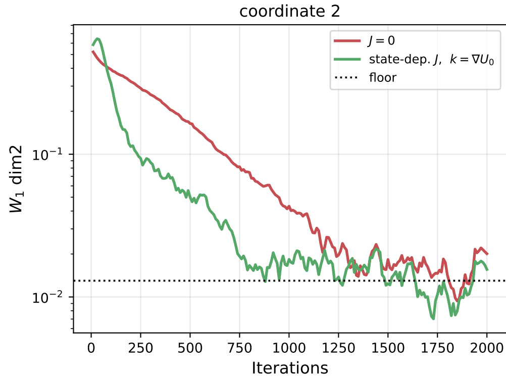
SCAD — J = 0 vs state-dependent J
