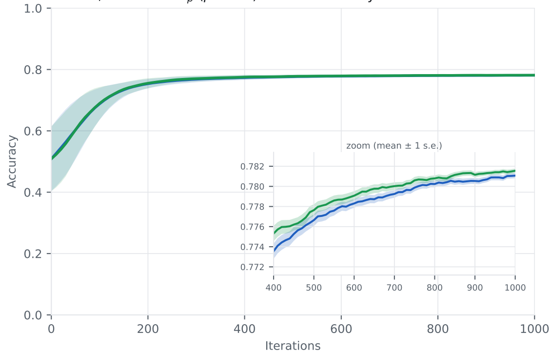
MAGIC, smoothed \ell_p ( p = 2.4 ) — test accuracy
