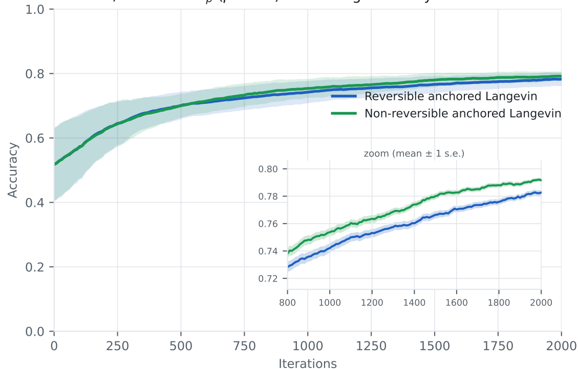
TITANIC, smoothed \ell_p ( p = 2.4 ) — training accuracy
