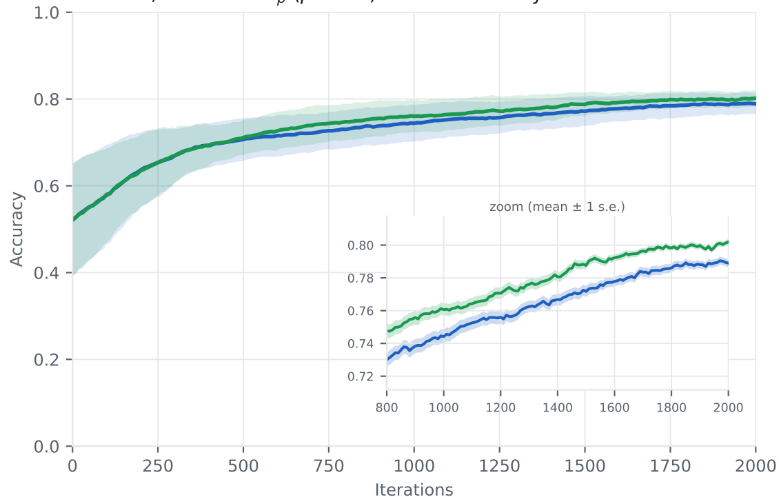
TITANIC, smoothed \ell_p ( p = 2.4 ) — test accuracy
