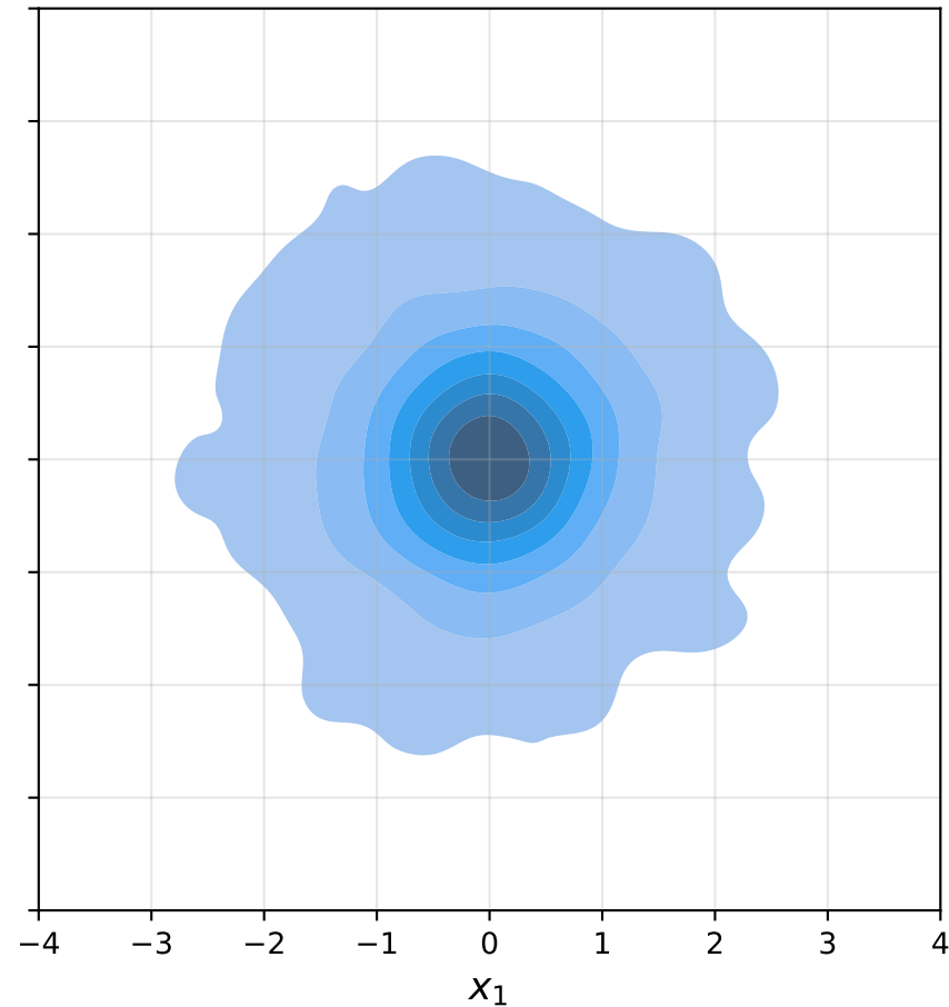
J_a, a = 2.0 (shown: |x| < 4.0 ; 99.1% of target mass)
