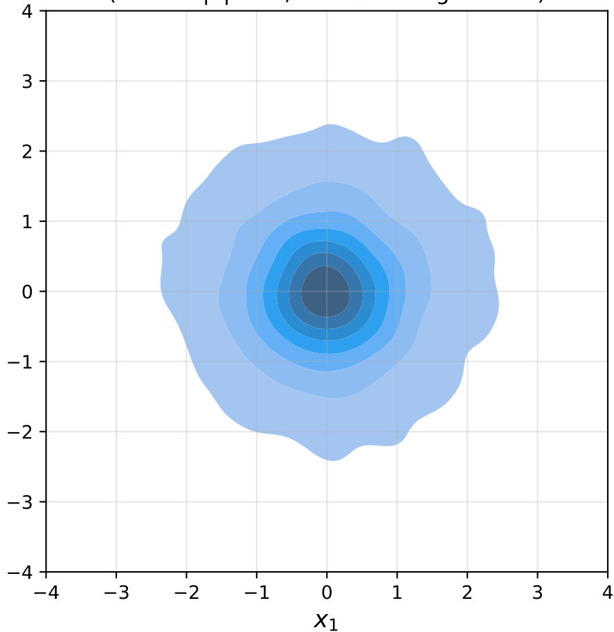
Target (exact draws) (shown: |x| < 4.0 ; 99.1% of target mass)
