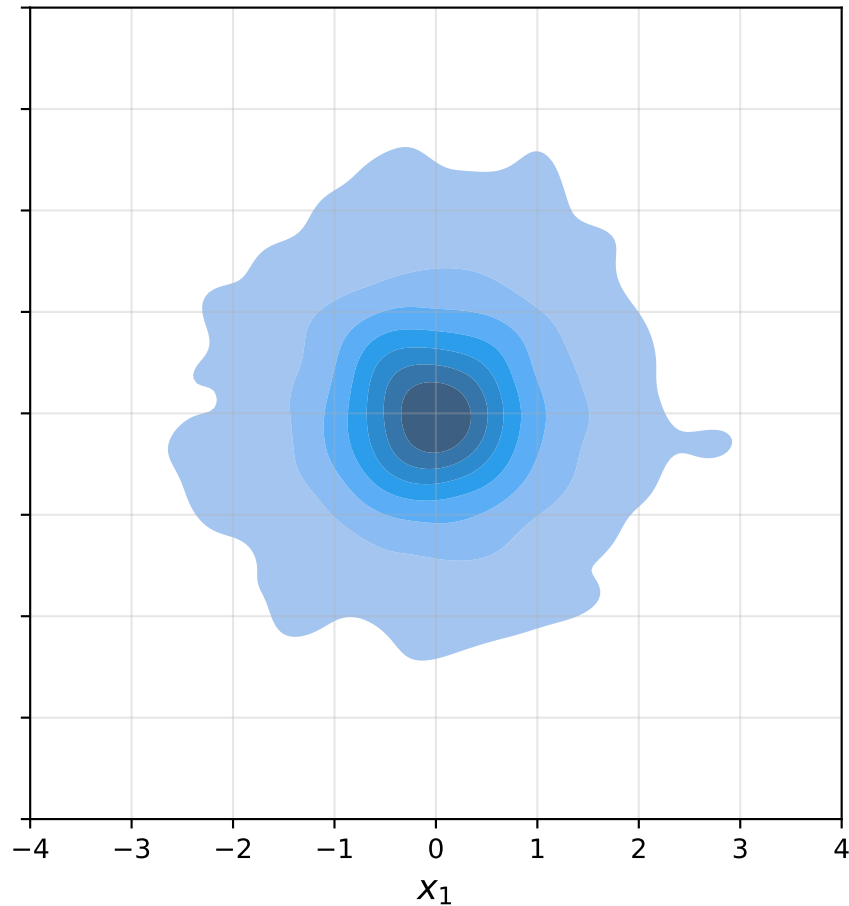
J = 0 (shown: |x| < 4.0 ; 99.1% of target mass)
