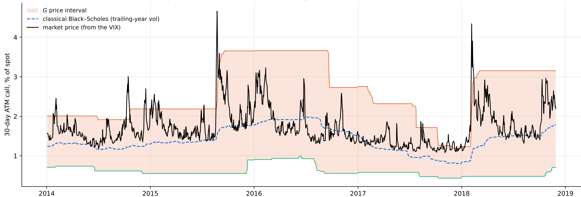
30-day at-the-money S&P 500 call: market against the classical price and the G interval
