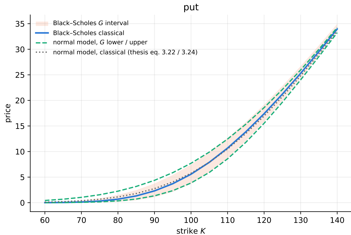
Lognormal (Black-Scholes) against normal (thesis, Bachelier) pricing, classical and G ; \sigma_m = 20.99 matched at the money
