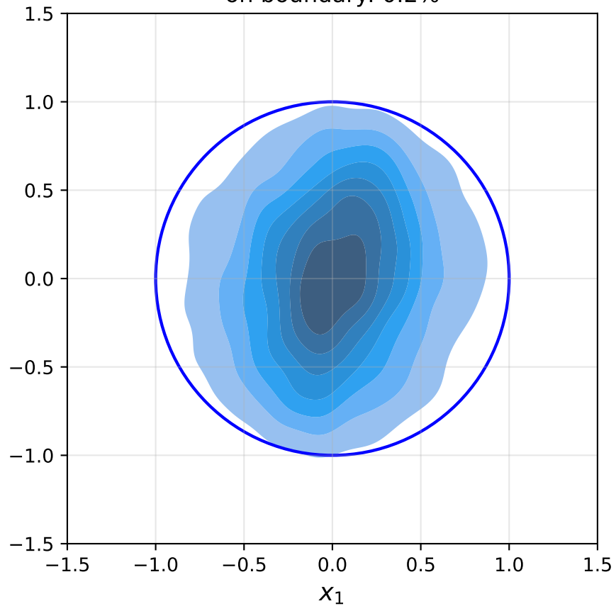
Target (rejection) on boundary: 0.2%
