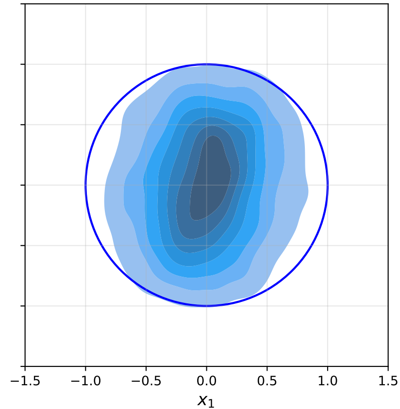
state-dependent J_s, s = 4.0 on boundary: 6.3%
