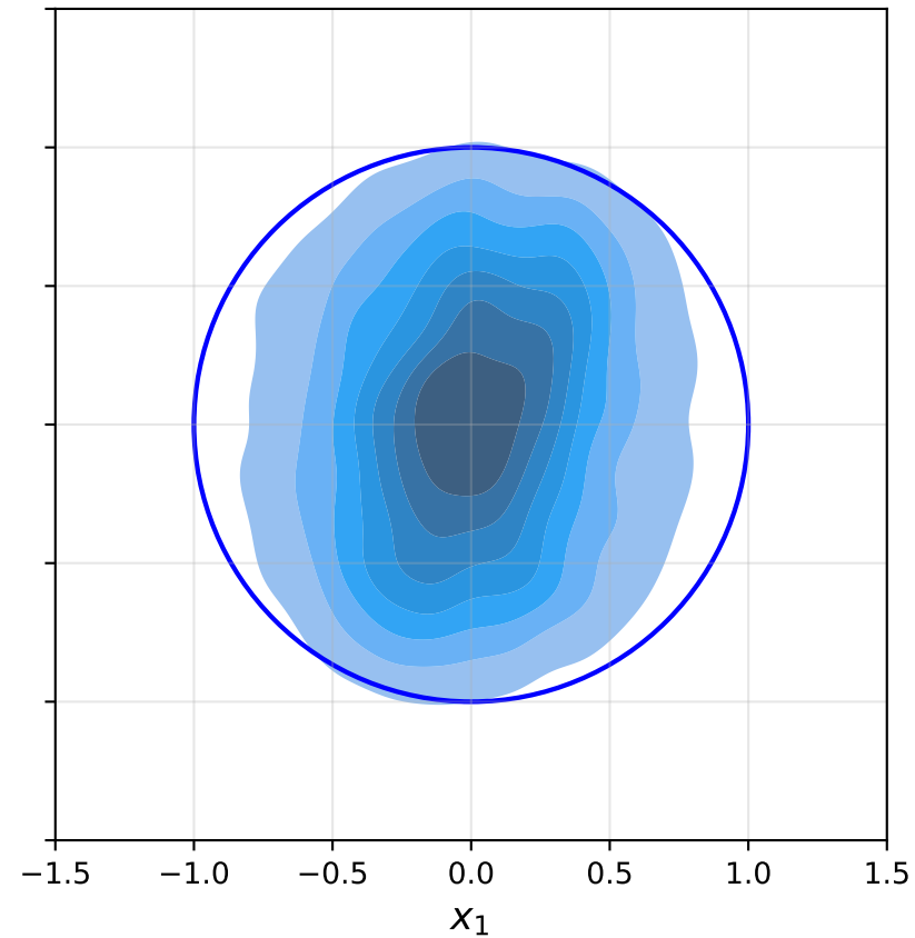
J = 0 on boundary: 6.1%
