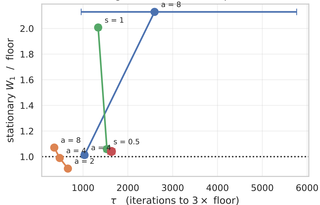
Target B: correlated \ell_1 Laplace
