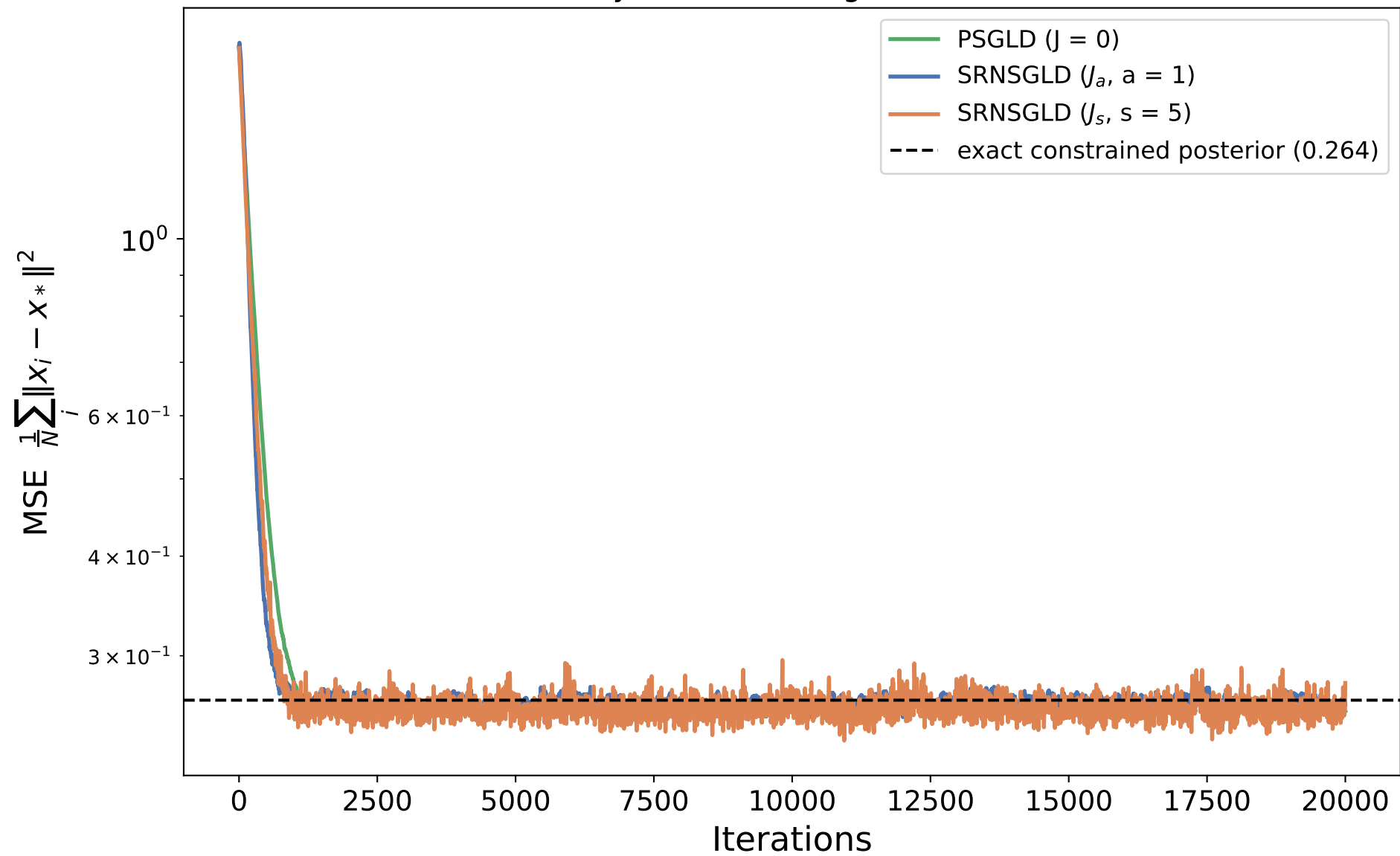
Constrained Bayesian linear regression, ball constraint
