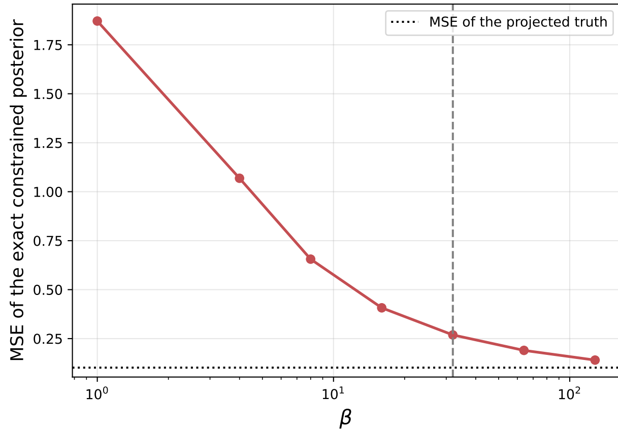
Choosing \beta : from uniform-on- K (small) to a point mass on \partial K (large)
