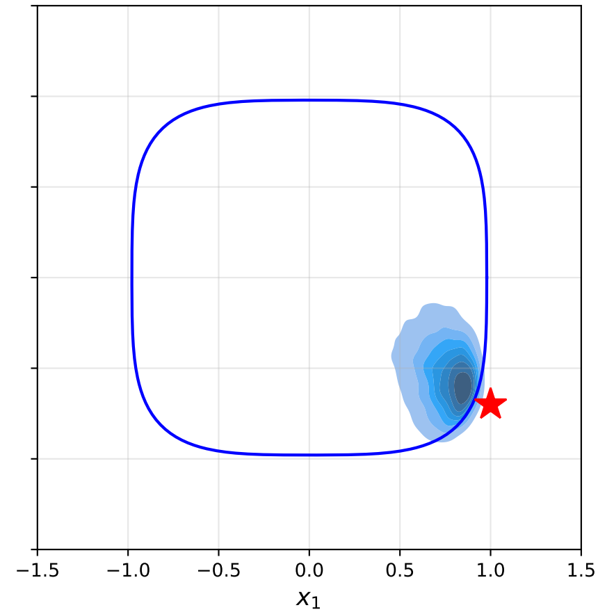
PSGLD ( J = 0 )
