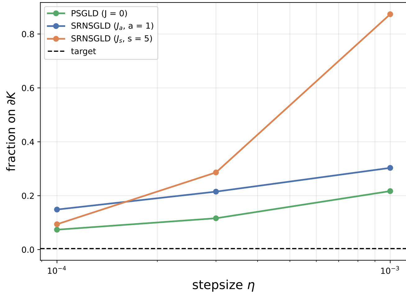
Tangential Euler steps overshoot: skew strength must be matched to the stepsize
