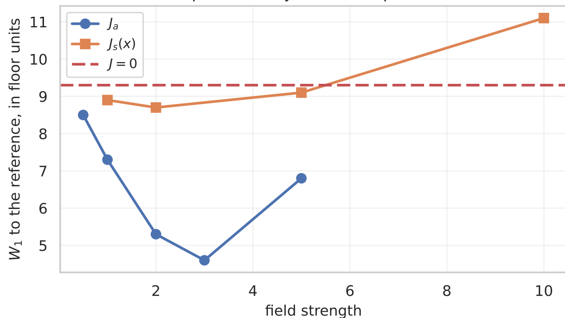
Telescope: accuracy of the sampled law itself
