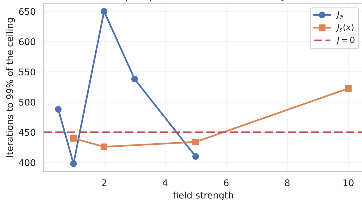
Telescope: speed, read off the accuracy curve
