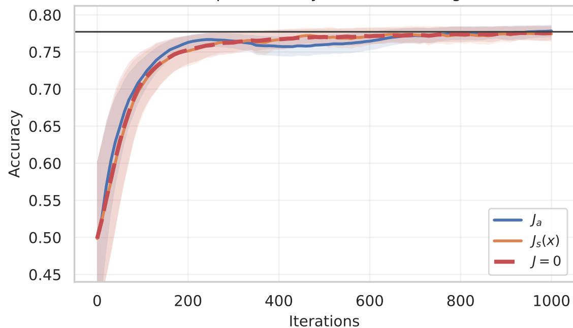
Telescope: accuracy over the training set
