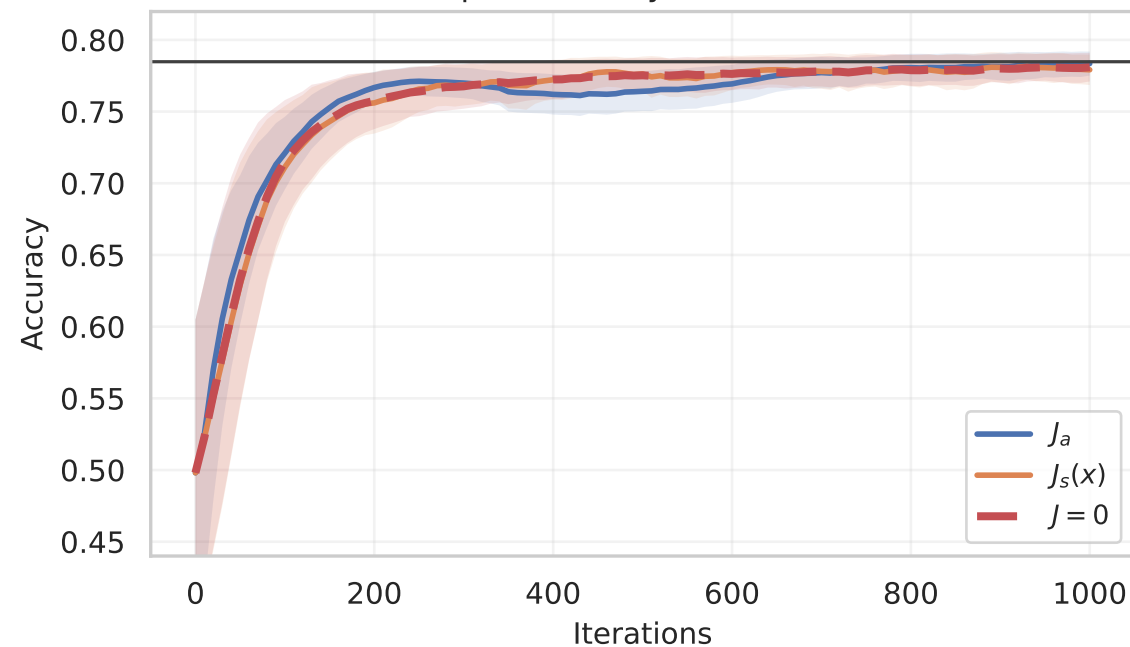
Telescope: accuracy over the test set
