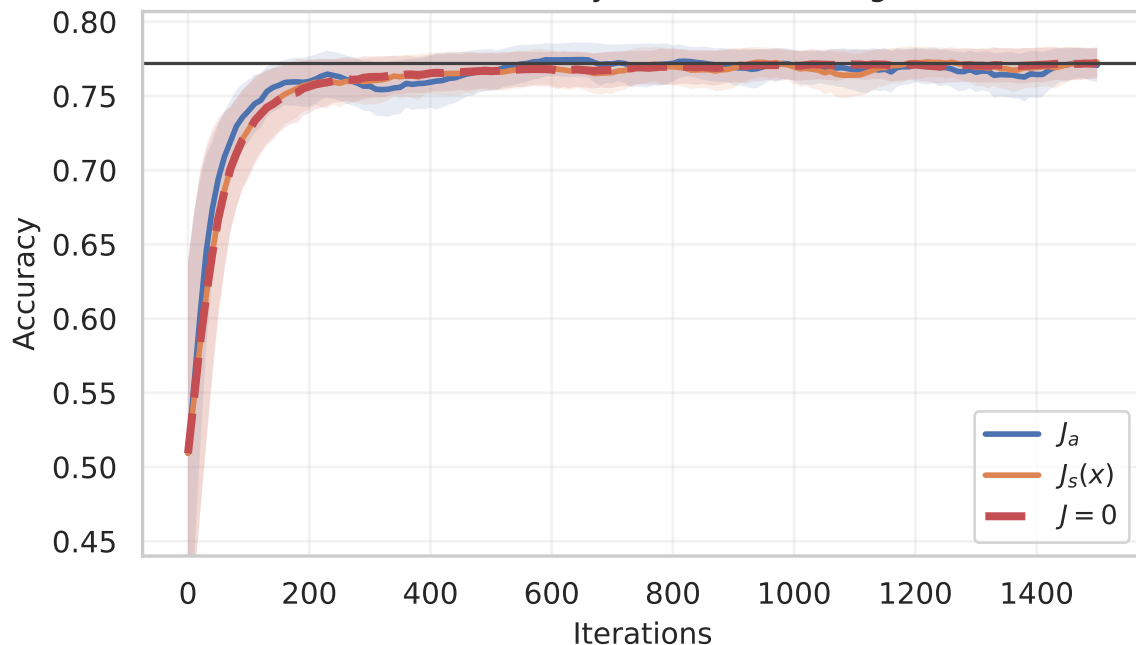
Titanic: accuracy over the training set
