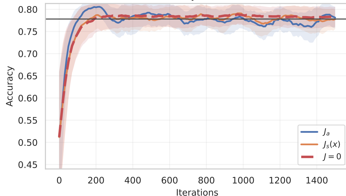
Titanic: accuracy over the test set
