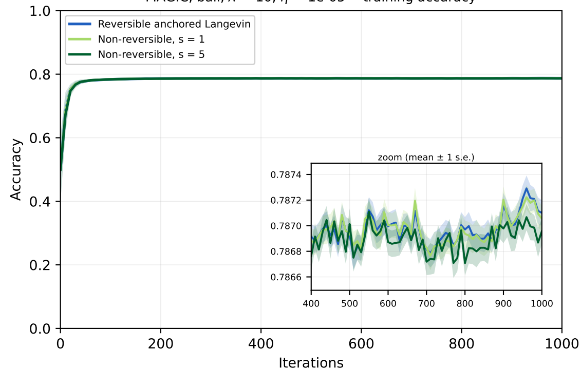
MAGIC, ball, \lambda = 10 , \eta = 1e-05 -- training accuracy
