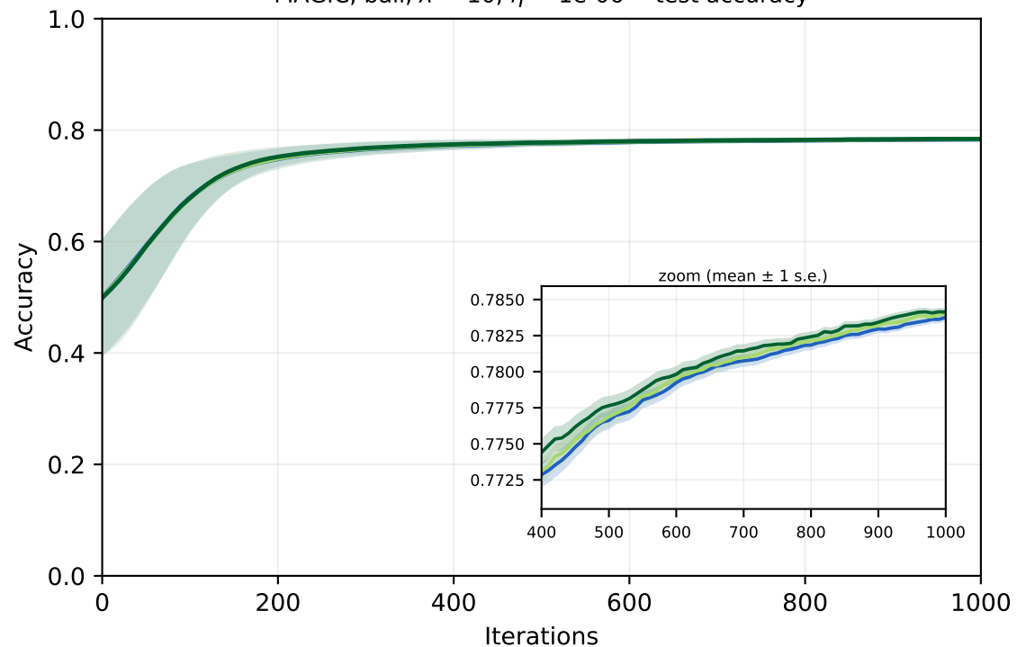
MAGIC, ball, \lambda = 10 , \eta = 1e-06 -- test accuracy
