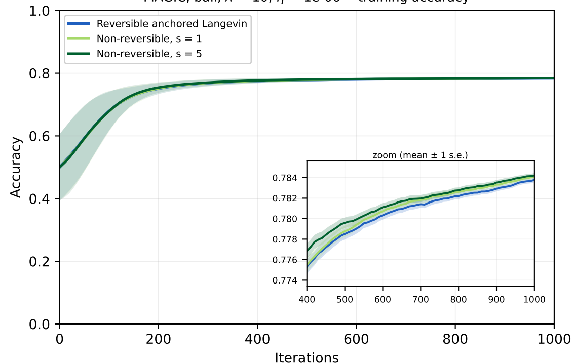
MAGIC, ball, \lambda = 10 , \eta = 1e-06 -- training accuracy
