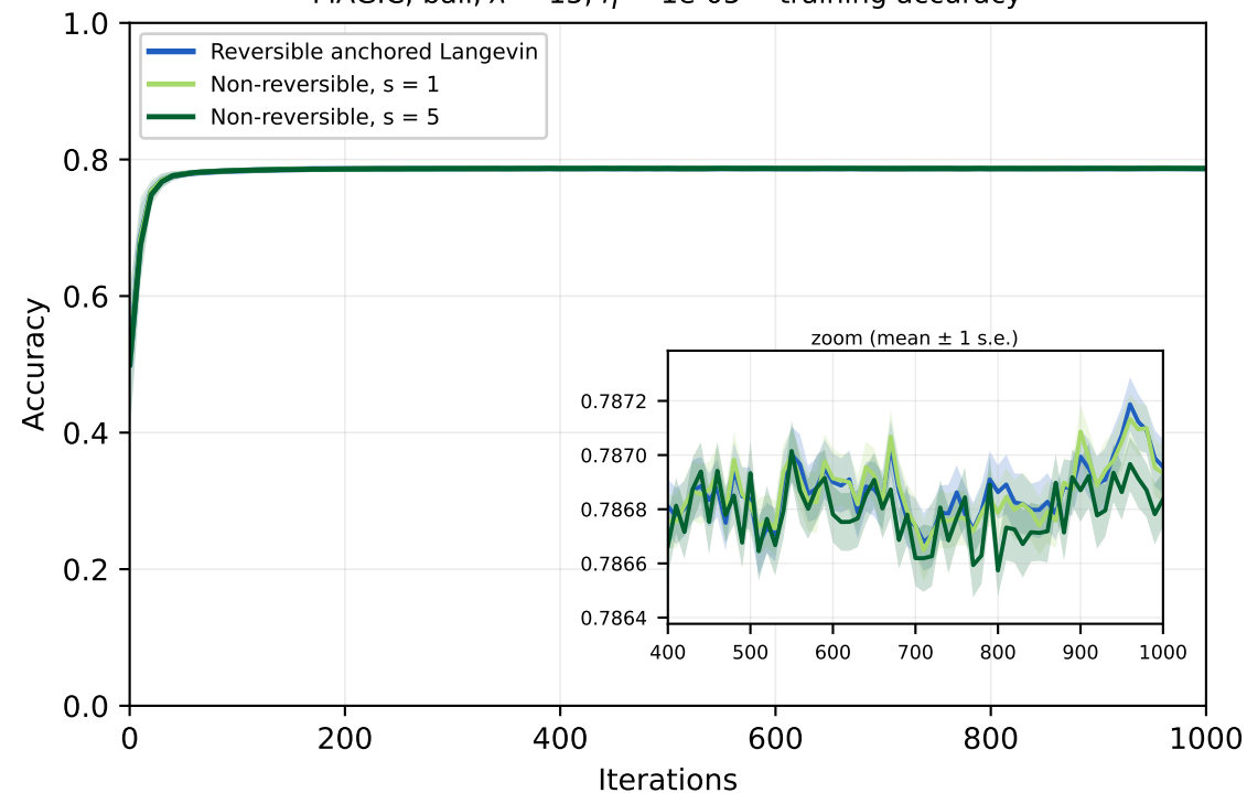
MAGIC, ball, \lambda = 15 , \eta = 1e-05 -- training accuracy
