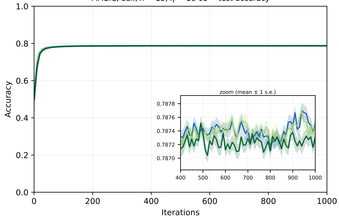
MAGIC, ball, \lambda = 15 , \eta = 1e-05 -- test accuracy
