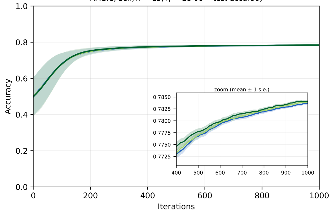
MAGIC, ball, \lambda = 15 , \eta = 1e-06 -- test accuracy
