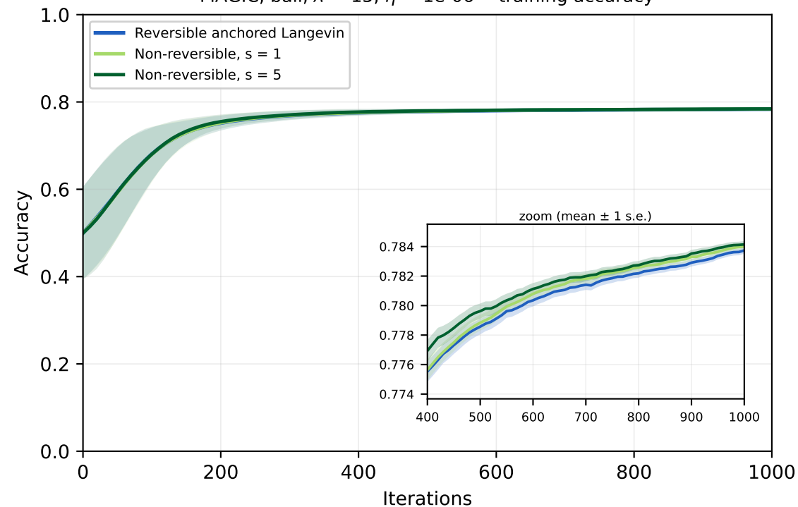
MAGIC, ball, \lambda = 15 , \eta = 1e-06 -- training accuracy
