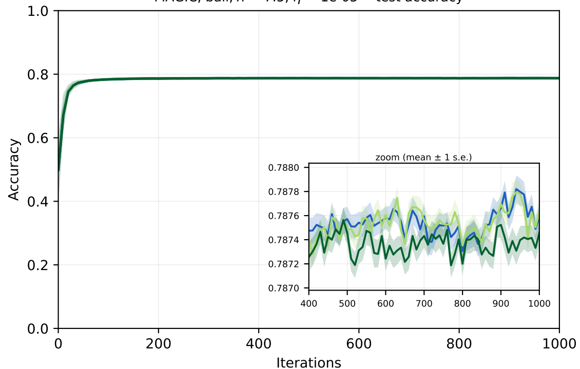
MAGIC, ball, \lambda = 7.5 , \eta = 1e-05 -- test accuracy
