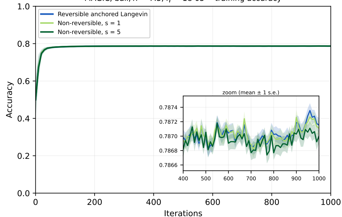
MAGIC, ball, \lambda = 7.5 , \eta = 1e-05 -- training accuracy
