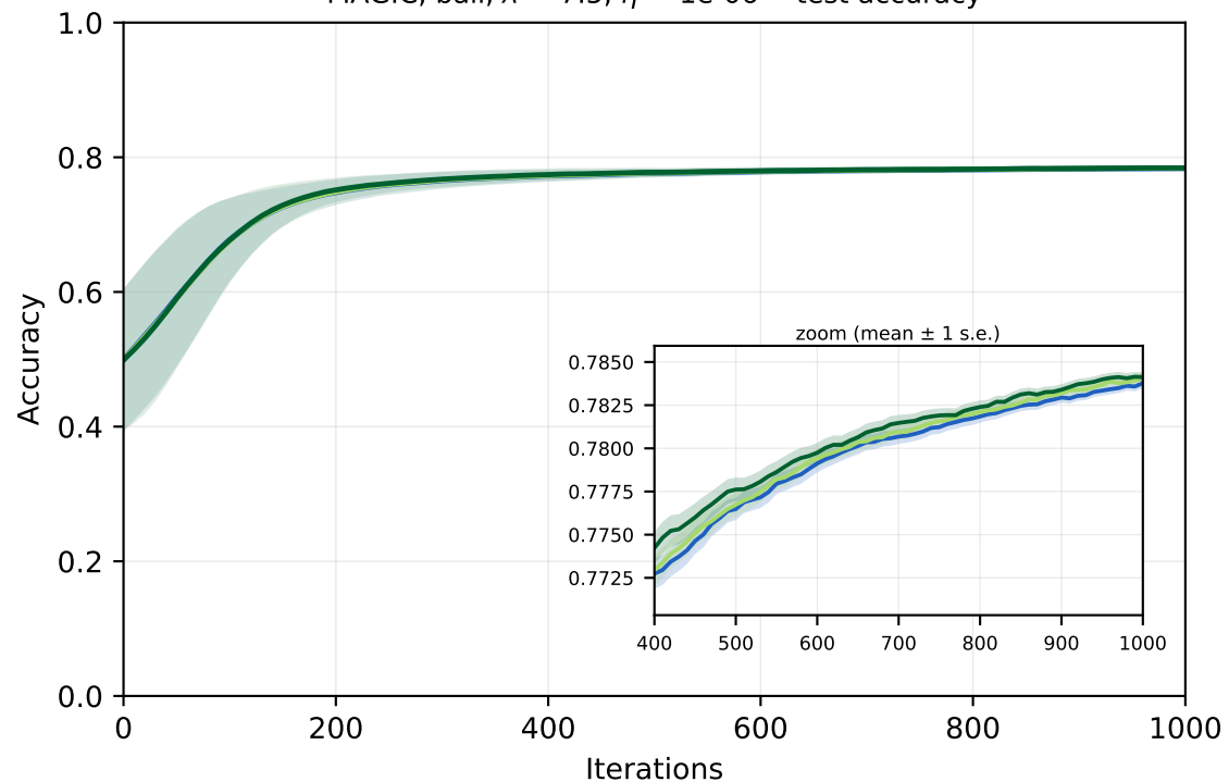
MAGIC, ball, \lambda = 7.5 , \eta = 1e-06 -- test accuracy
