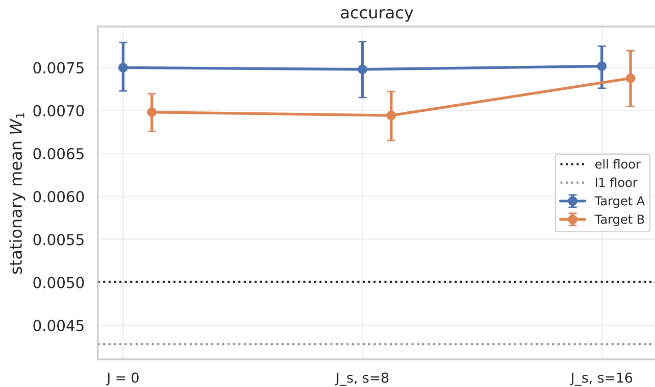
J_s against J = 0 : speed and accuracy at each strength
