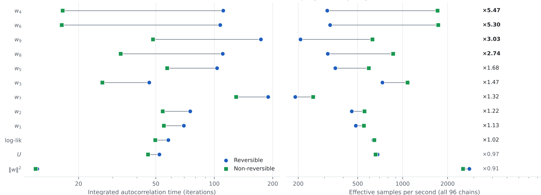
Autocorrelation time (lower is better)
