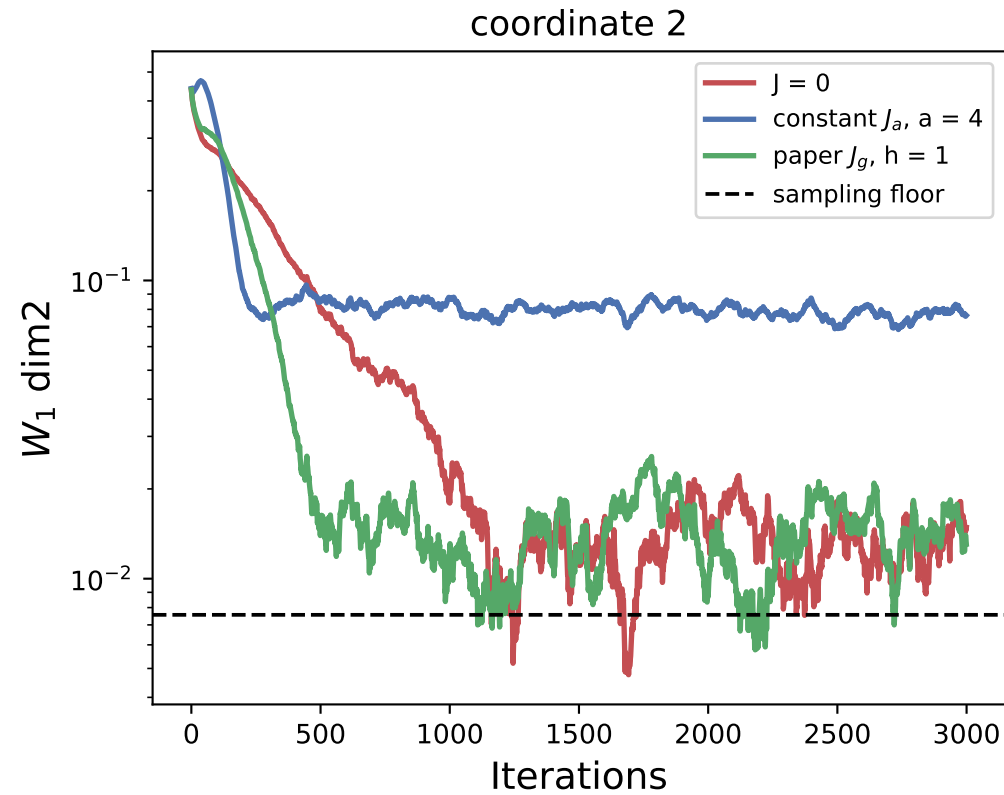
Smoothed \ell_p ball ( p = 4 , \varepsilon = 0.2 , \lambda = 1 ): the paper's J_g
